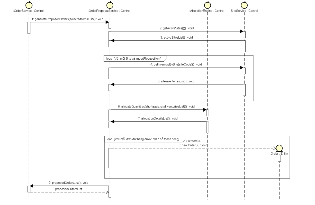
sd SequenceDiagram_004
